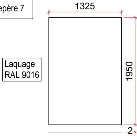
Ech: 1/40
